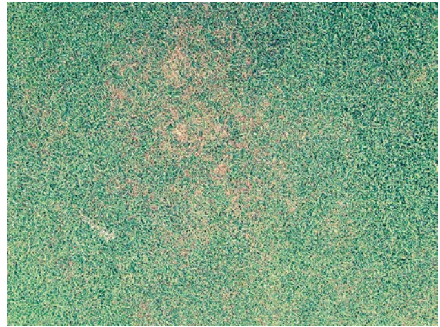
Figure 5-28. Anthracnose basal rot in the cool, wet season attacking mostly creeping bentgrass.
